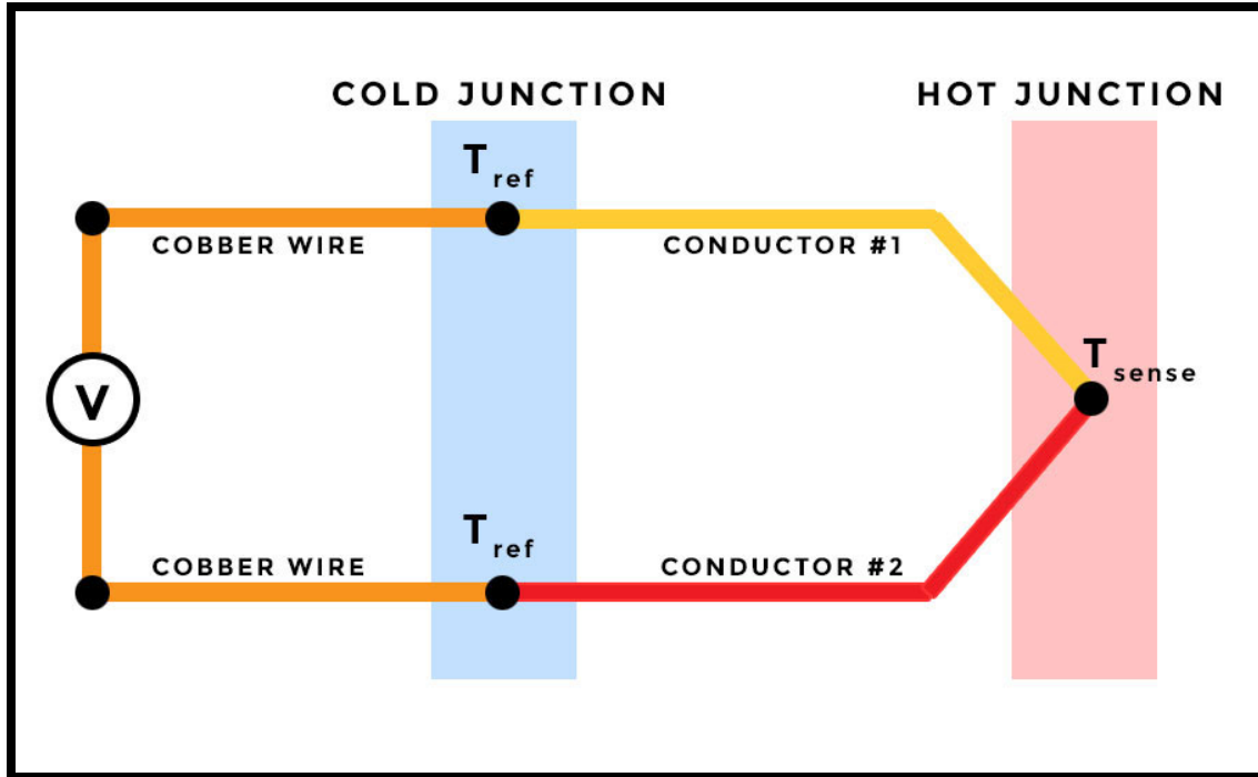
Figure 16: Thermocouple Diagram
